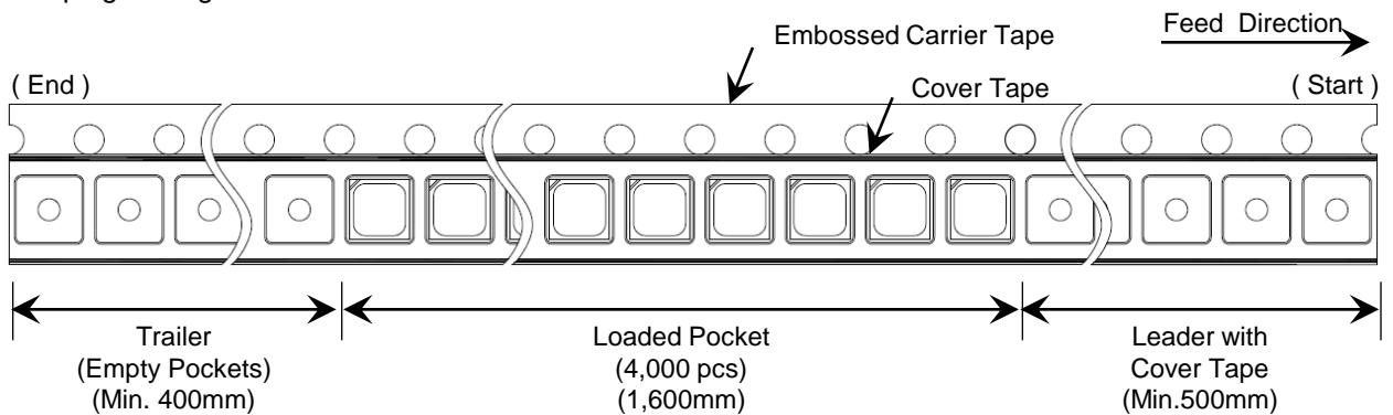
Taping Arrangement
