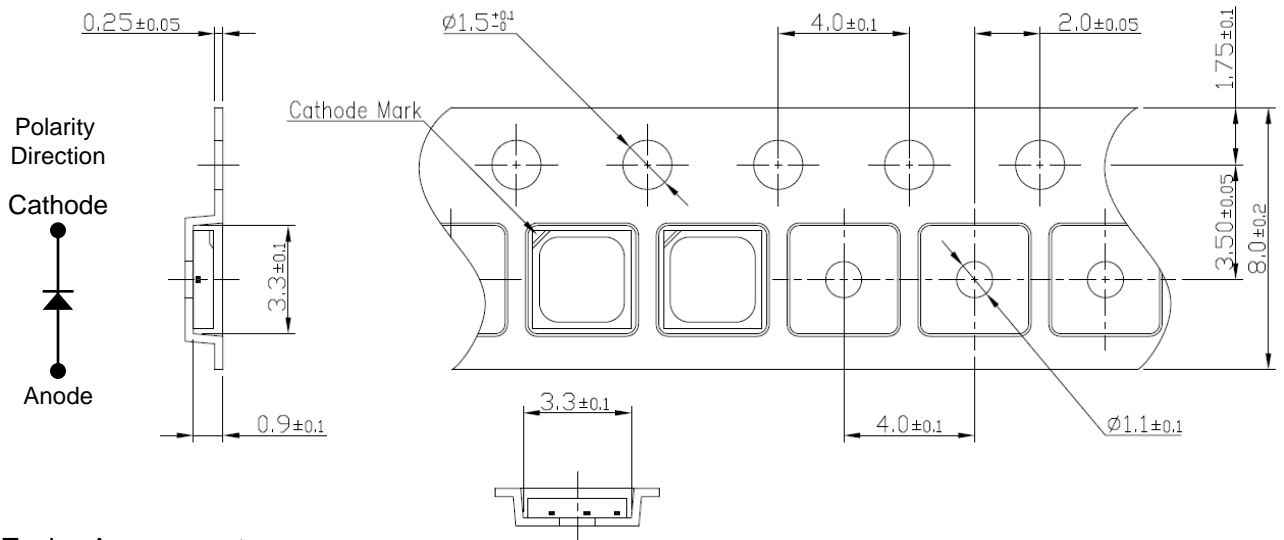
Taping Arrangement
