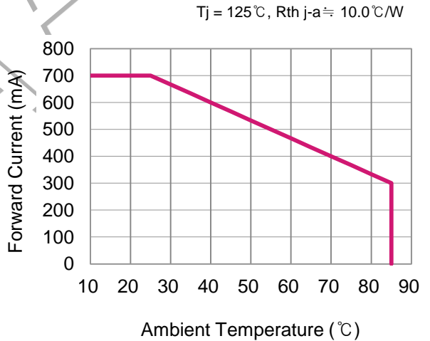
■ Derating Curve
